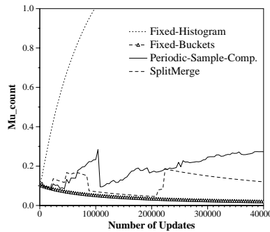
Figure 7: \mu_{count} errors (equi-depth histograms)
