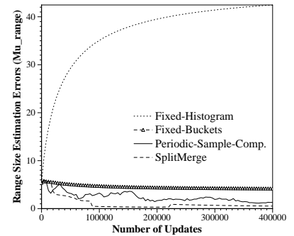
Figure 8: \mu_{range} errors (equi-depth histograms)
